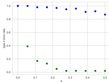
type II error rate for m = 40 t -tests of linear relationship with (blue) and without (green) Bonferroni correction
